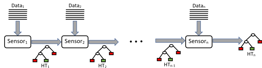
Figure 2. Incremental learning with Hoeffding trees.
